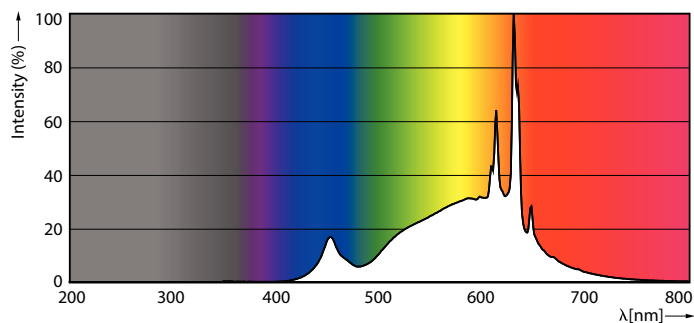
Spectral Power Distribution Colour - MAS VLE LEDBulb D5.9-60W E27 927
