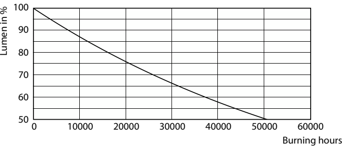
Lumen Maintenance Diagram - TForce Core LED HPL 13W E27 840 FR
