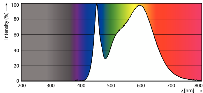
Spectral Power Distribution Colour - CorePro LEDbulb ND 8-60W A60 E27 840
