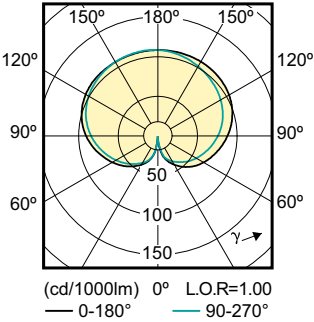
Light Distribution Diagram – LED classic 60W A60 E27 WW FR ND 1CT/10
