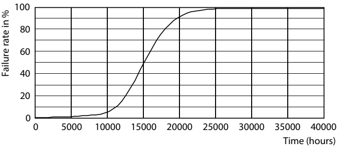
Life Expectancy Diagram - CorePro LEDbulb ND 4.9-40W A60 E27 840
