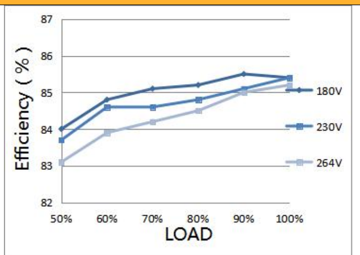
Fig.6 Efficiency-Load curve
