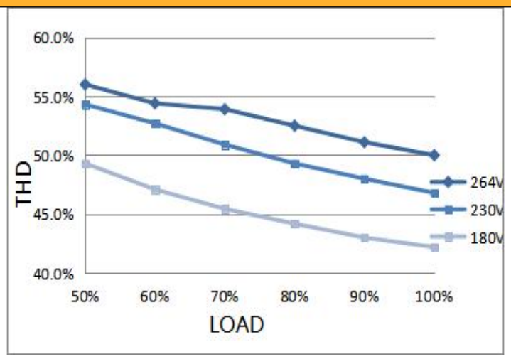
Fig.5 Total harmonic distortion curve ( THD )
