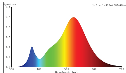
LED-Retrofit-Lamps 2700K
