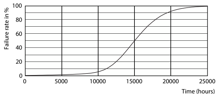
Life Expectancy Diagram - Corepro LEDspot 3.5-35W GU10 830 36D
