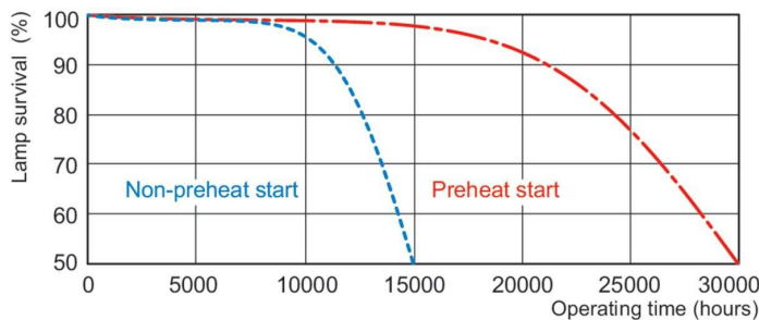
Life Expectancy Diagram - MASTER TL5 HO 39W/827 SLV/40
