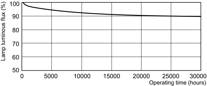
Lumen Maintenance Diagram - MASTER TL5 HO 39W/827 SLV/40
