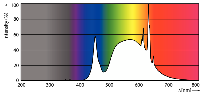
Spectral Power Distribution Colour - MAS LEDCandleND2.3-40W E14 840B35 CLG UE
