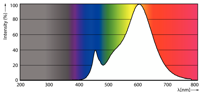
Spectral Power Distribution Colour - CorePro lustre ND 5-40W E14 827 P45
